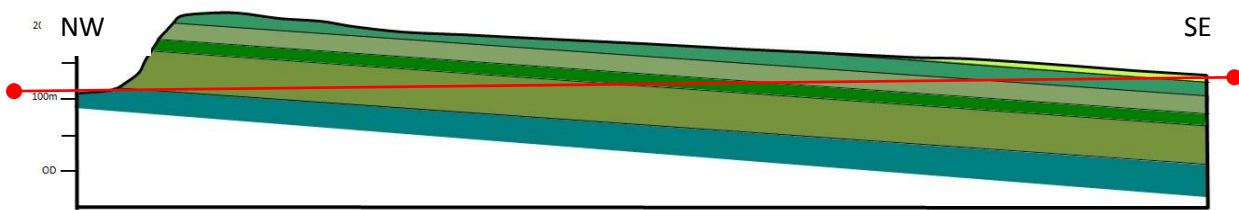
Figure 2: Schematic geological cross section through the Chilterns. Different chalk formations dip gently to the south, forming the northern rim of the London Basin. The red line shows how any proposed rail route would tunnel/cut from younger to older chalk passing from the southeast to the northwest.
